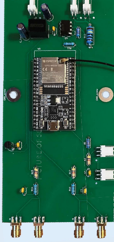
Figure 5-1: A picture of the PCB design of the Sensor Unit
