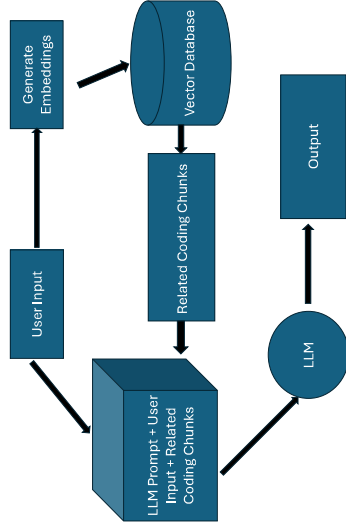
Figure 2: High Level Architecture for RAG Model
