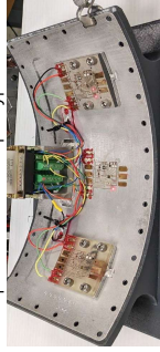
Example of printed electronics placed on a dewar pinout https://ntrs.nasa.gov/citations/20220008696 https://ntrs.nasa.gov/citations/20220014746
