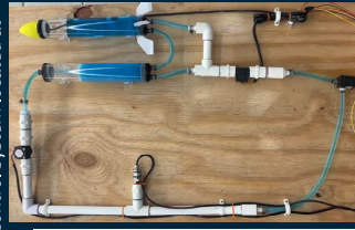
Fig 2: Testbench
